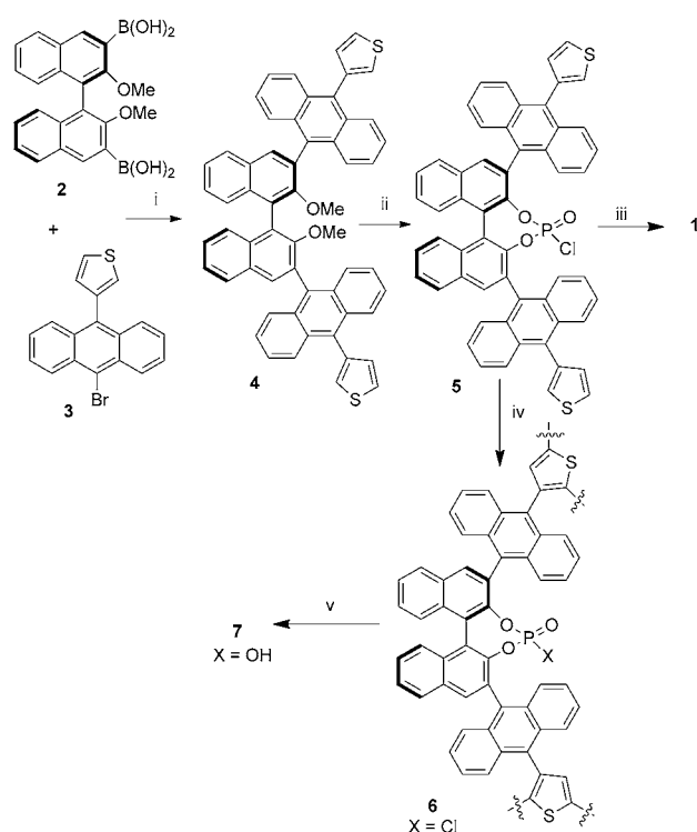
Scheme 2. Synthesis of the polymer network. Conditions: i) [\text{Pd}(\text{PPh}_3)_4] , \text{K}_2\text{CO}_3 , THF/ \text{H}_2\text{O} , 80^\circ\text{C} ; ii) a) \text{BBr}_3 , \text{CH}_2\text{Cl}_2 , b) poly(4-vinyl pyridine), \text{POCl}_3 , \text{CH}_2\text{Cl}_2 ; iii) THF, 1 M HCl, RT; iv) \text{FeCl}_3 , toluene, acetonitrile; v) aqueous HCl.
